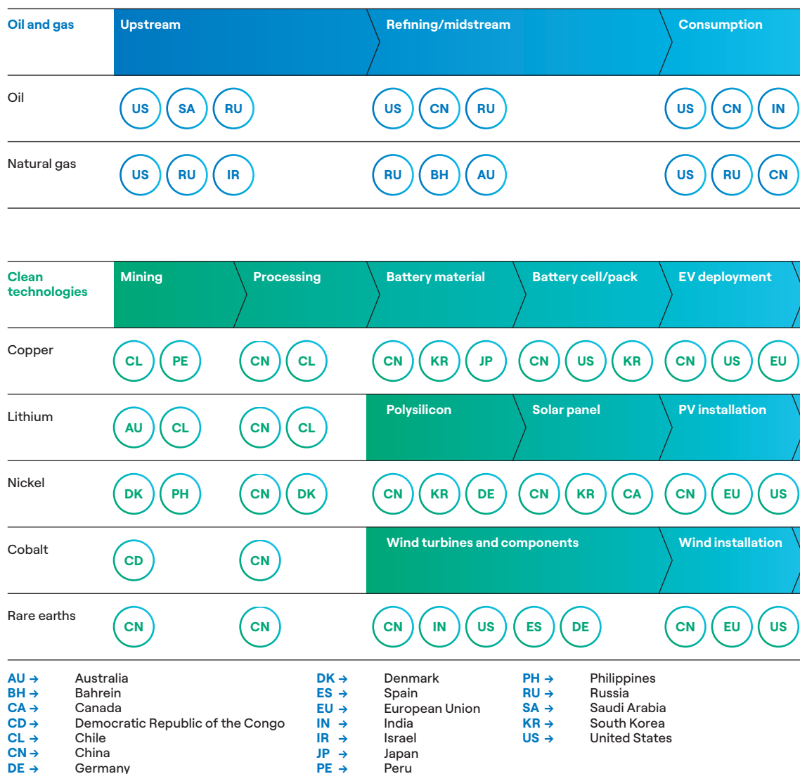
FIG 13 → Indicative supply chains of oil and gas and selected clean energy technologies
