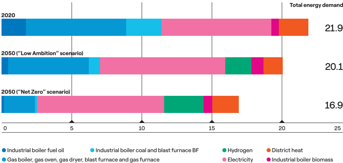
FIG 35 → Energy demand in industry by technology in Italy, 2020–2050 (Mtoe)
