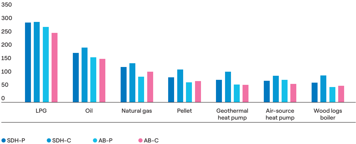
FIG 41 → Levelized Cost of Heat for domestic heating according to different scenarios, 2022 (€/MWh)
