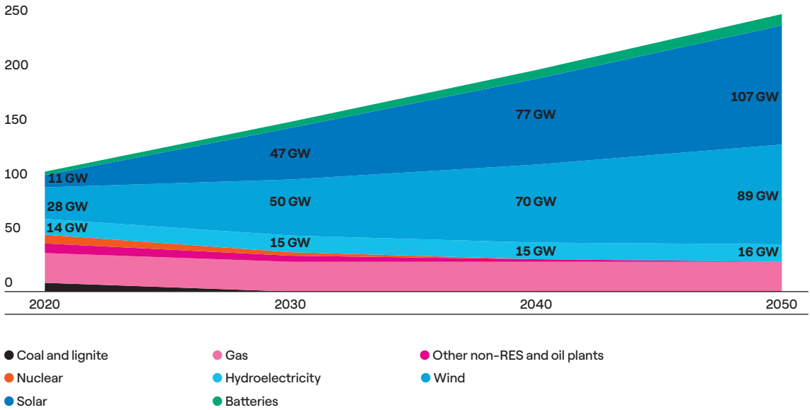
FIG 21 → Capacity mix by technology in the “Low Ambition” scenario in Spain, 2020–2050 (GW)
