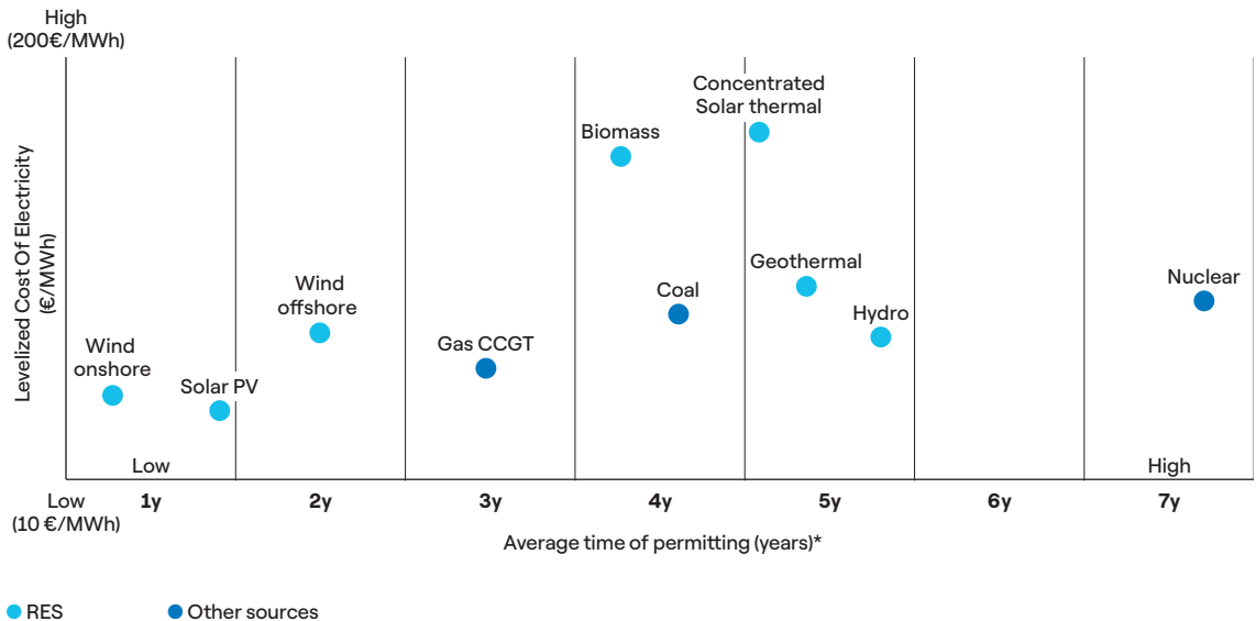
FIG 15 → Median LCOE by technology in the European Union (€/MWh)
