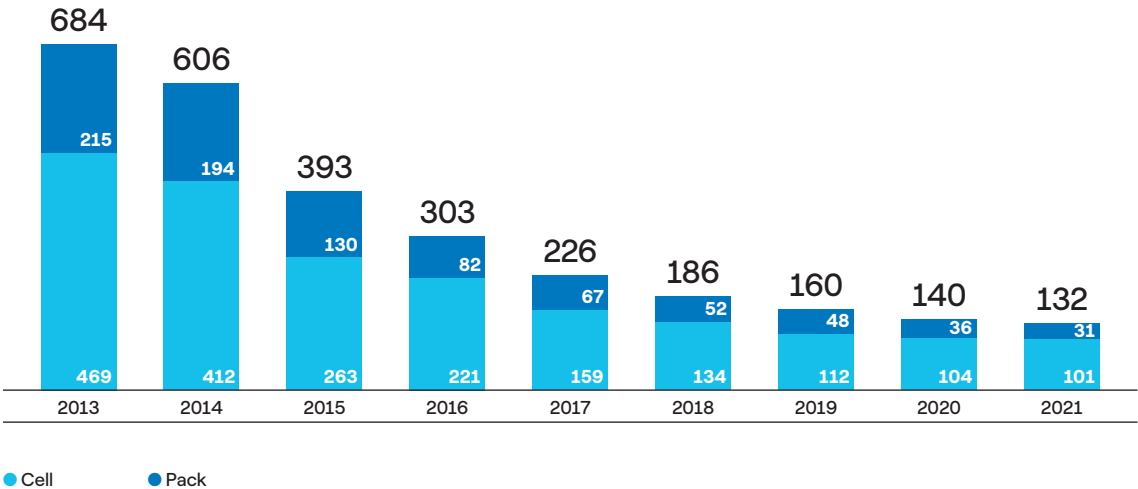
FIG 27 → Average lithium-ion cell and pack price, 2013–2021 (USD/kWh, 2021 constant prices)
