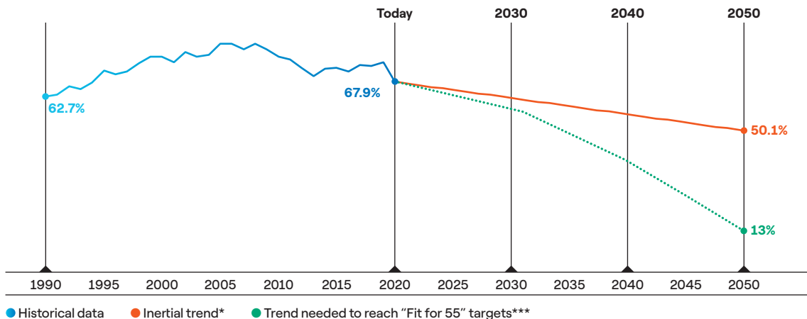
FIG 35 → Energy dependence in Spain, 1990–2050 E (% values)
