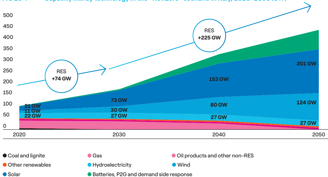
FIG 20 → Capacity mix by technology in the “Net Zero” scenario in Italy, 2020–2050 (GW)
