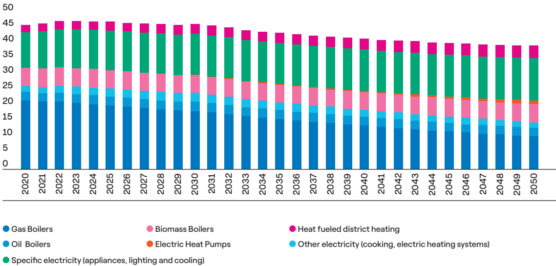
FIG 43 → Energy demand of buildings in the “Low Ambition” scenario in Italy, 2020–2050 (Mtoe)
