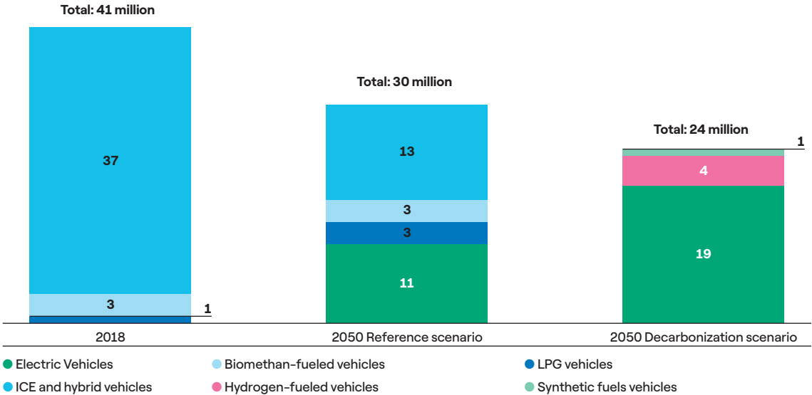
FIG 6 → Total vehicles fleet by energy vector in 2018 and in Reference and Decarbonization scenarios in Italy, 2018 and 2050 (millions of units)
