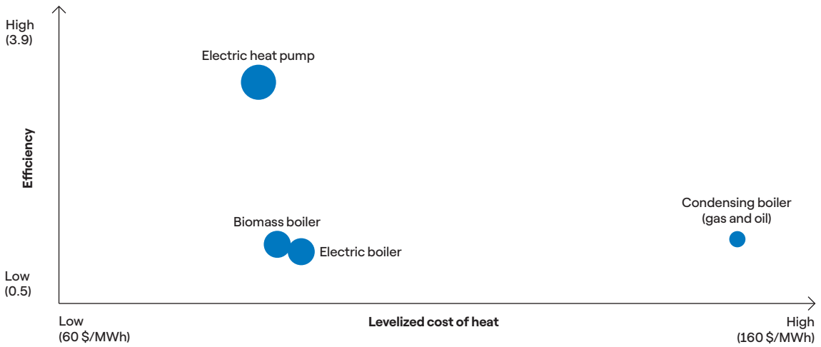
FIG 42 → Assessment of residential sector technologies by cost of heat (X axis: $/MWh) and efficiency at European level (Y axis: energy input/energy output), 2021
