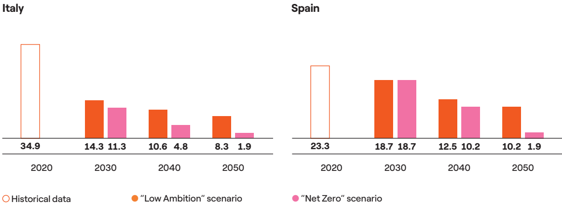
FIG 20 → Evolution of the gas intensity of GDP index in Italy (left chart) and Spain (right chart) in the “Low Ambition” and “Net Zero” scenario, 2020, 2030, 2040 and 2050 (toe per million Euros of GDP)
