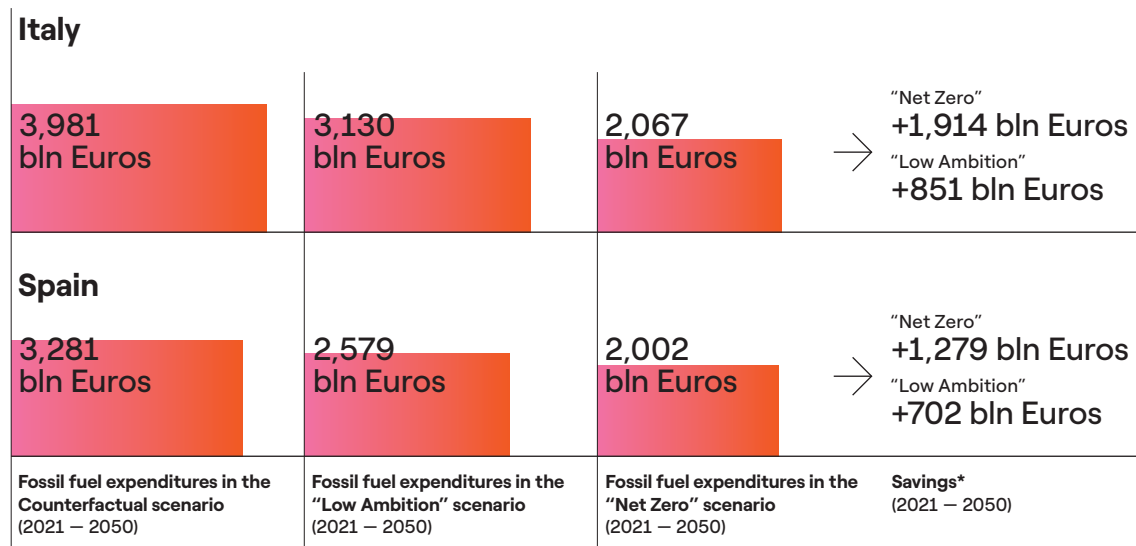
FIG 19 → Fossil fuel expenditures in the “Low Ambition”, “Net Zero” and Counterfactual scenarios in Italy and Spain, 2021–2050 (billion Euros)
