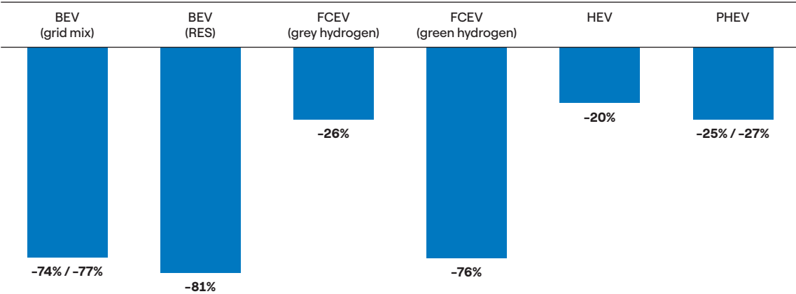
FIG 28 → Life cycle greenhouse gas (GHG) emissions of selected vehicles (% reduction compared to Internal Combustion Engines)
