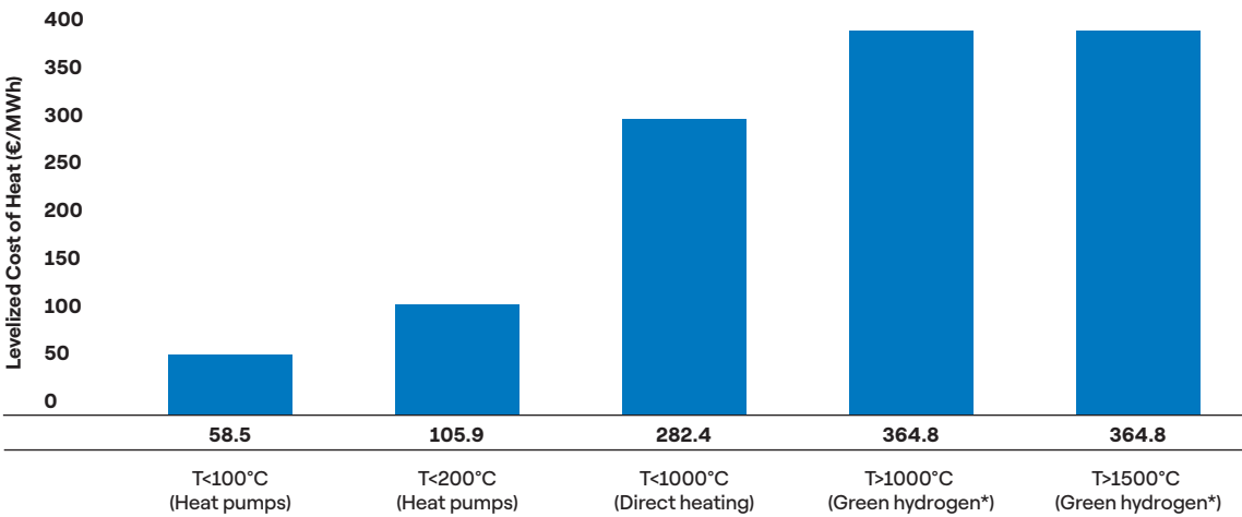
FIG 33 → Estimated Levelized Cost of Heat for electric appliances compared to fossil fuel technologies, 2030 (€/MWh)
