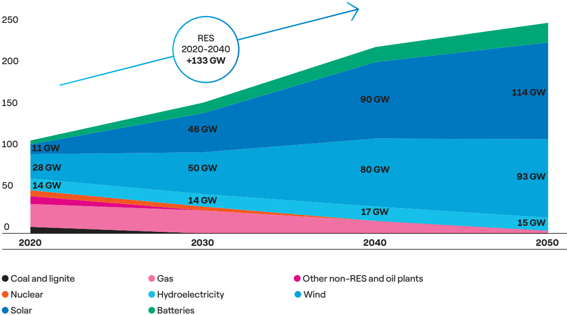
FIG 22 → Capacity mix by technology in the “Net Zero” scenario in Spain, 2020–2050 (GW)
