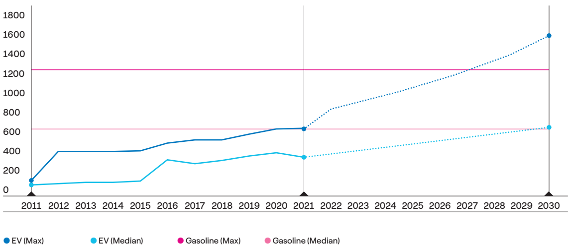
FIG 26 → Forecast of median and maximum range autonomy of Electric Vehicles, 2011–2030 E (km)
