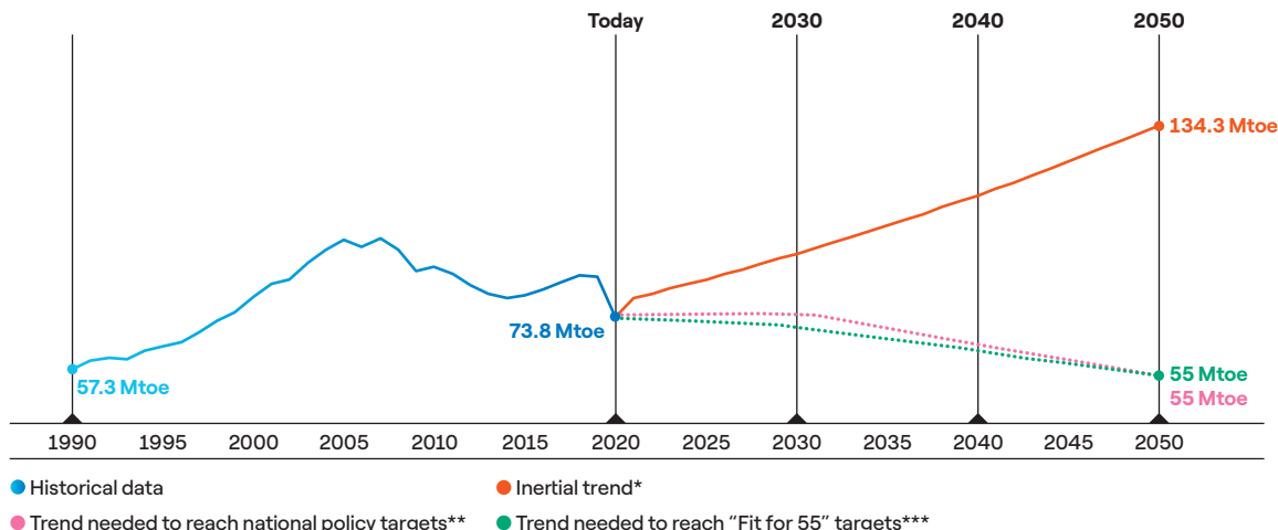
FIG 17 → Energy efficiency in Spain, 2005–2050 E (Mtoe)
