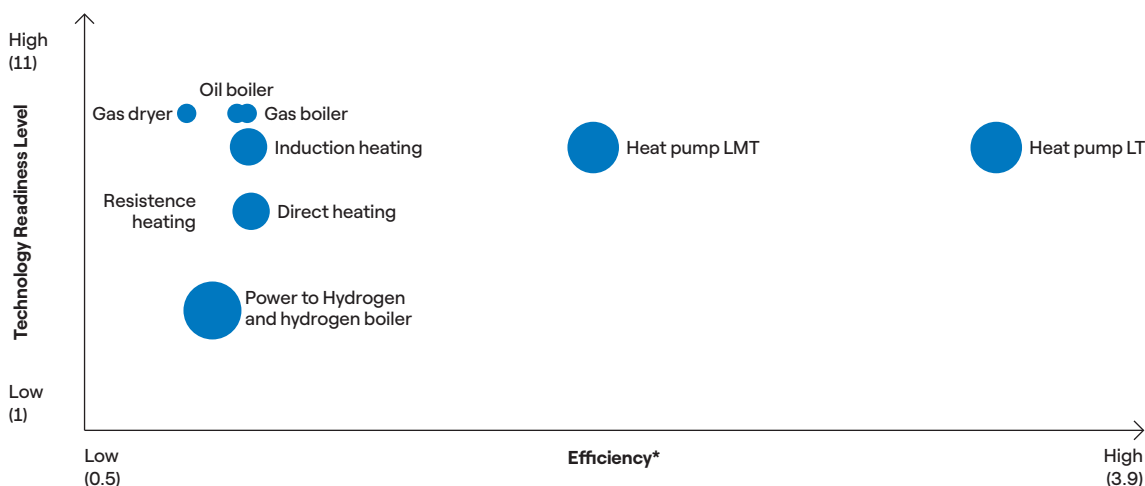
FIG 34 → Assessment of technologies in industrial sector by efficiency (X axis: energy input/energy output) and TRL at European level (Y axis: values from 1 to 11), 2021
