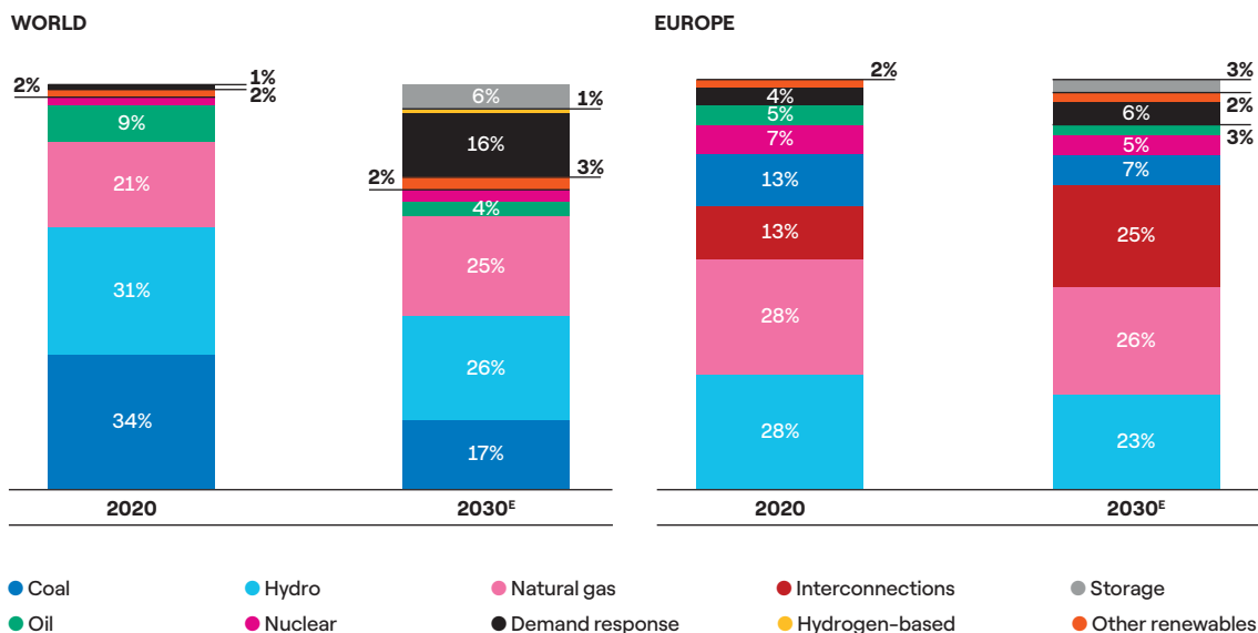
FIG 48 → Electricity system flexibility by source at global and European level, 2020 and 2030 E (% values)
