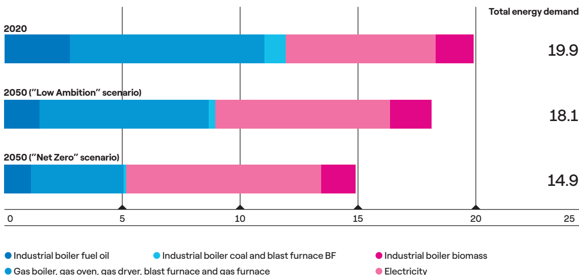
FIG 36 → Energy demand in industry by technology in Spain, 2020–2050 (Mtoe)
