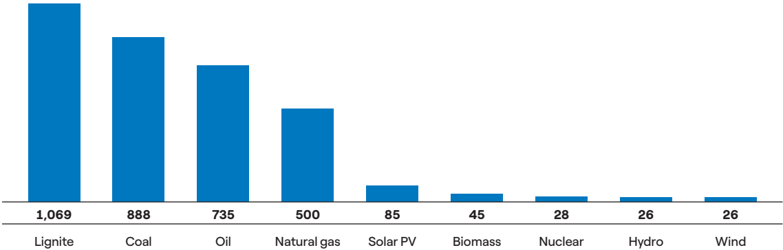
FIG 16 → GHG emission intensity during the life cycle of electricity production by technology, 2021 or the latest available data (tonnes of CO 2 -eq. per GWh)
