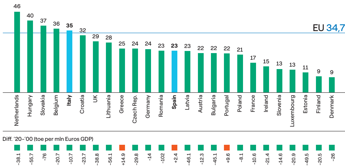
FIG 28 → Gas intensity of GDP index in EU27 Countries, UK and Europe, 2020 (absolute values, toe per mln Euros of GDP)
